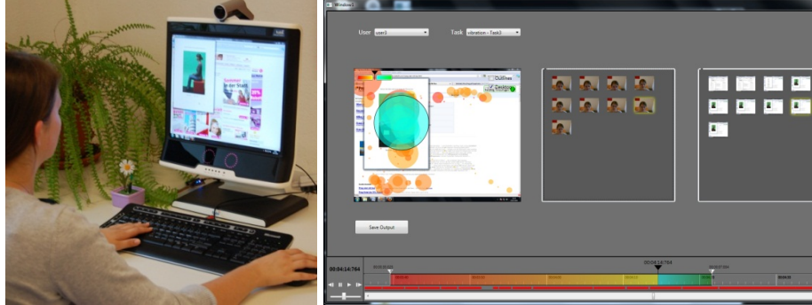
Fig. 5. ( left ) The apparatus of the user study including the eye-tracking LCD of Tobii. ( right ) The custom analyzing tool allows a better analysis of how participants react to an interrupt. Capturing the participants' screen augmented with the gazing plot helped us to analyze better the results.
