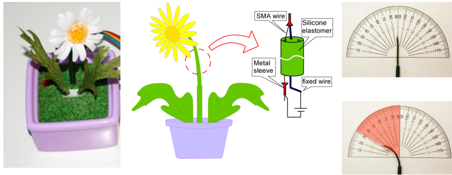
Fig. 4. ( left ) The bending plant represents the office worker’s posture. ( center ) The image of the plant and detail of the actuator which consists of a fixed and a SMA wire. ( right ) The bending shape of the actuator without the bloom ( top : without power, bottom : with power).
